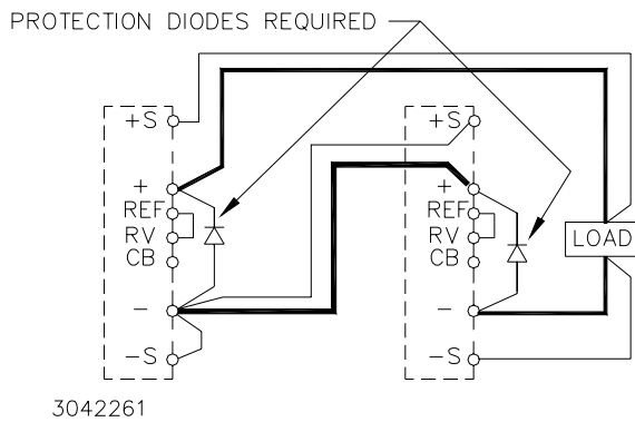
FIGURE 12. SERIES CONNECTION
