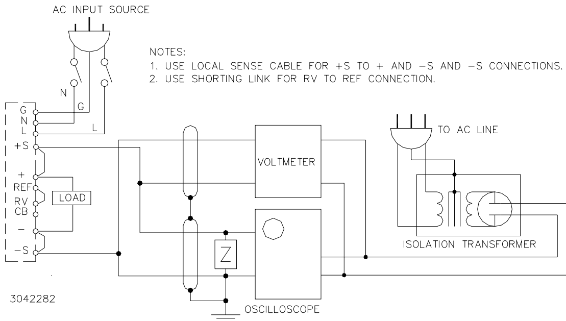
FIGURE 13. FUNCTIONAL CHECKOUT
